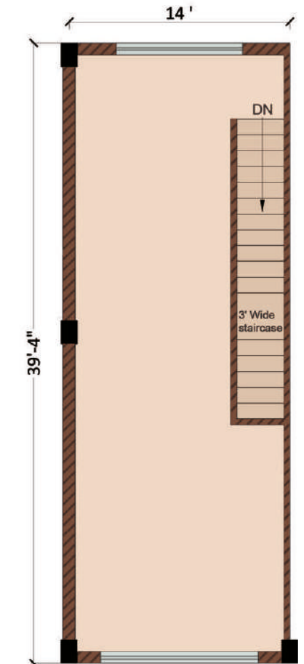
First Floor Plan Covered Area: 550 sq.ft. Floor to Floor Height: 15 ft.
